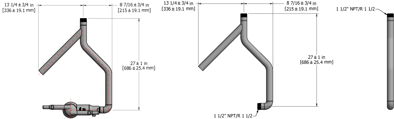
Adapter with HydroWhirl Orbitor 2 x 10
