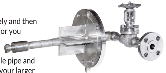
WTZ Lance with Inlet Valve and Gussets
